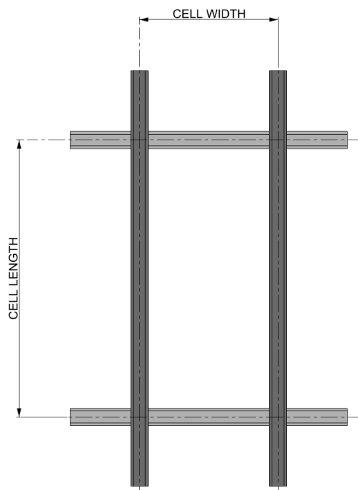
GRYD Cell Dimensions
